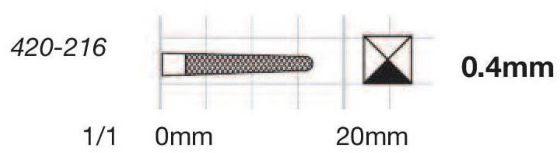
381 - M 6450 Neivert Needle Holder, Serrated, TC, 13cm
